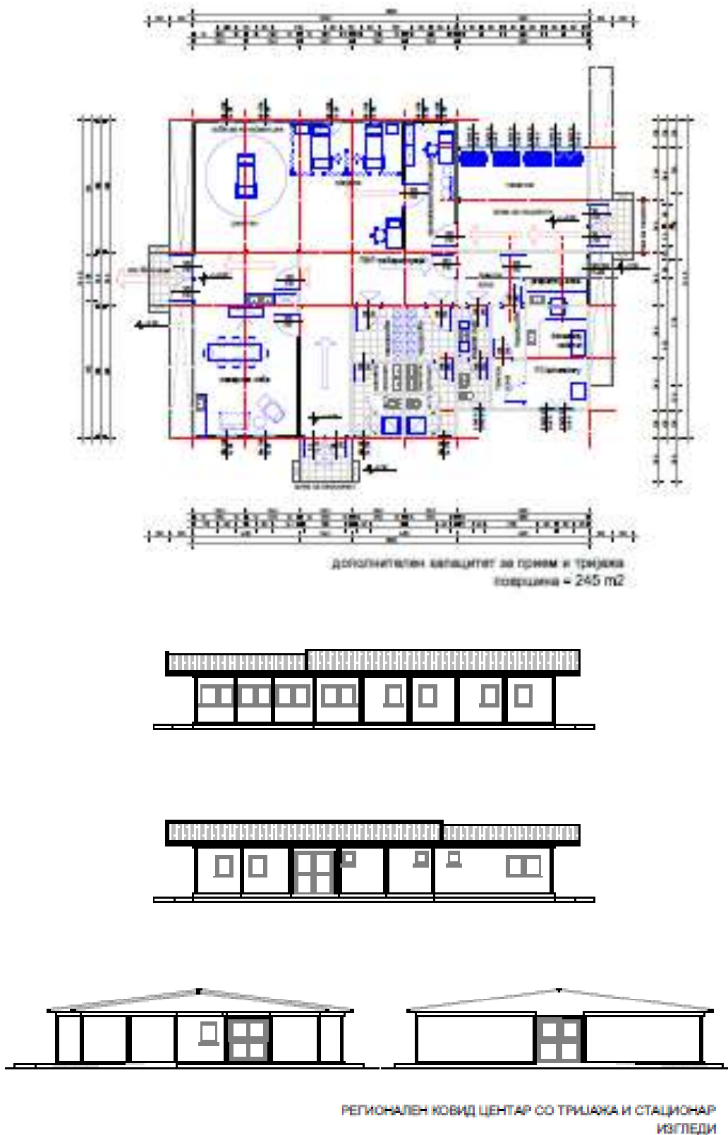
Figure 3 The look of the extended construction of the mobile hospital in Municipality of Skopje - Kozle
