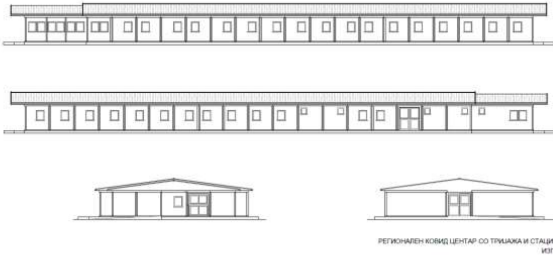
Figure 3 The look of the extended construction of the mobile hospital in Municipality of Ohrid
